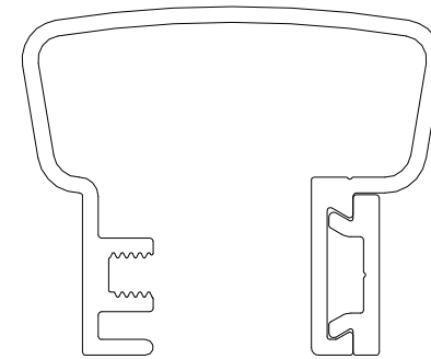
#9005 TOP RAIL WITH #9007 SCREW COVER
