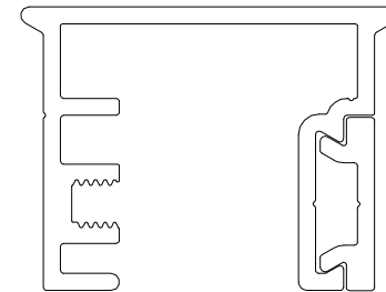
#9003 BOTTOM RAIL WITH #9007 SCREW COVER
